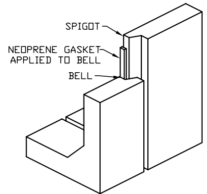
JOINT DETAIL
