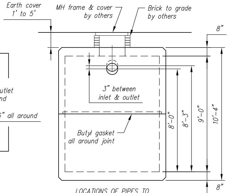
LOCATIONS OF PIPES TO BE PROVIDED BY CONTRACTOR
