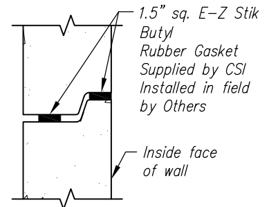
JOINT DETAIL
