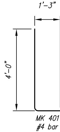
BENDING SCHEDULE
