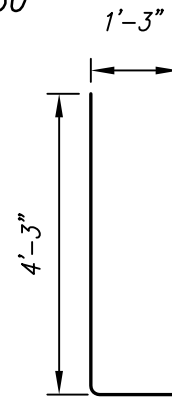
MK 401 #4 bar BENDING SCHEDULE
