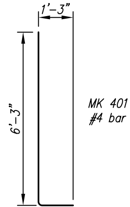
BENDING SCHEDULE
