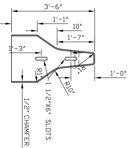
END VIEW
